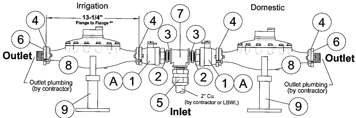
Detail with both meters installed
